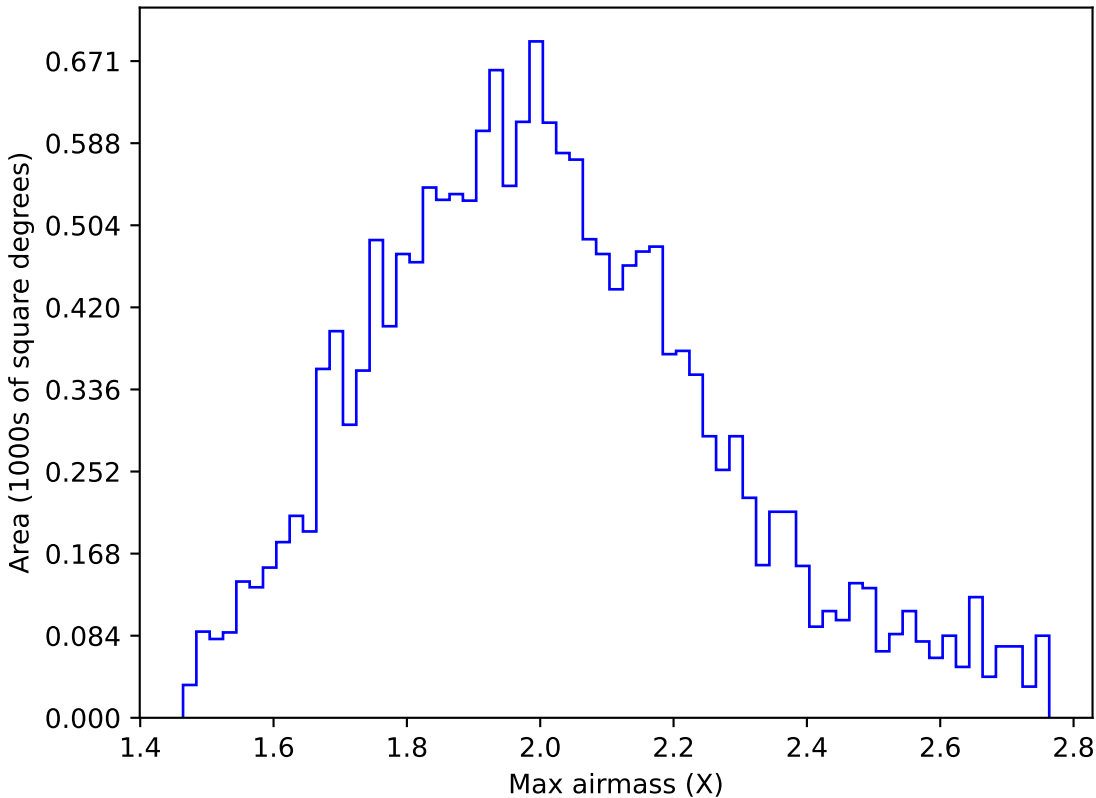
weather_cloudso2v3.4_10yrs WFD g band: Max airmass
