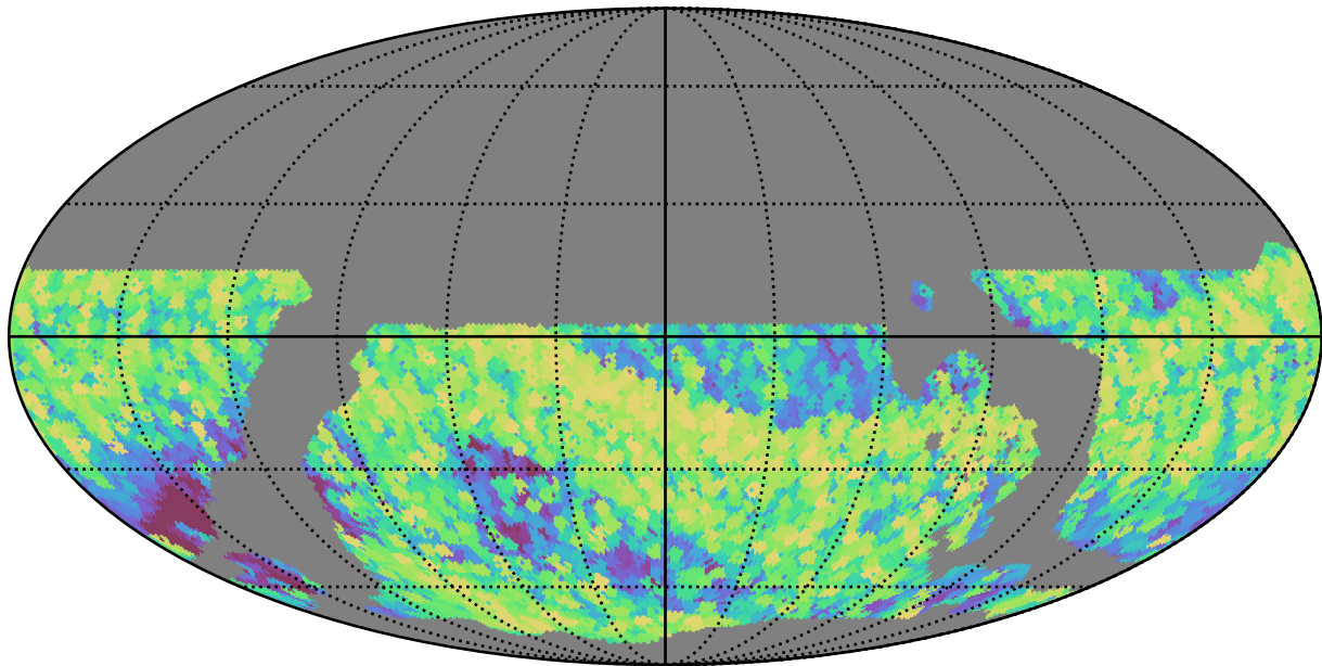
weather_cloudso2v3.4_10yrs WFD all bands: Max airmass
