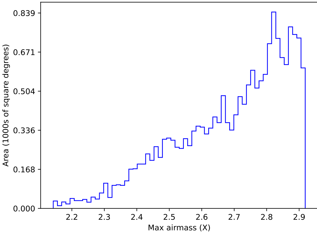
weather_cloudso2v3.4_10yrs WFD all bands: Max airmass
