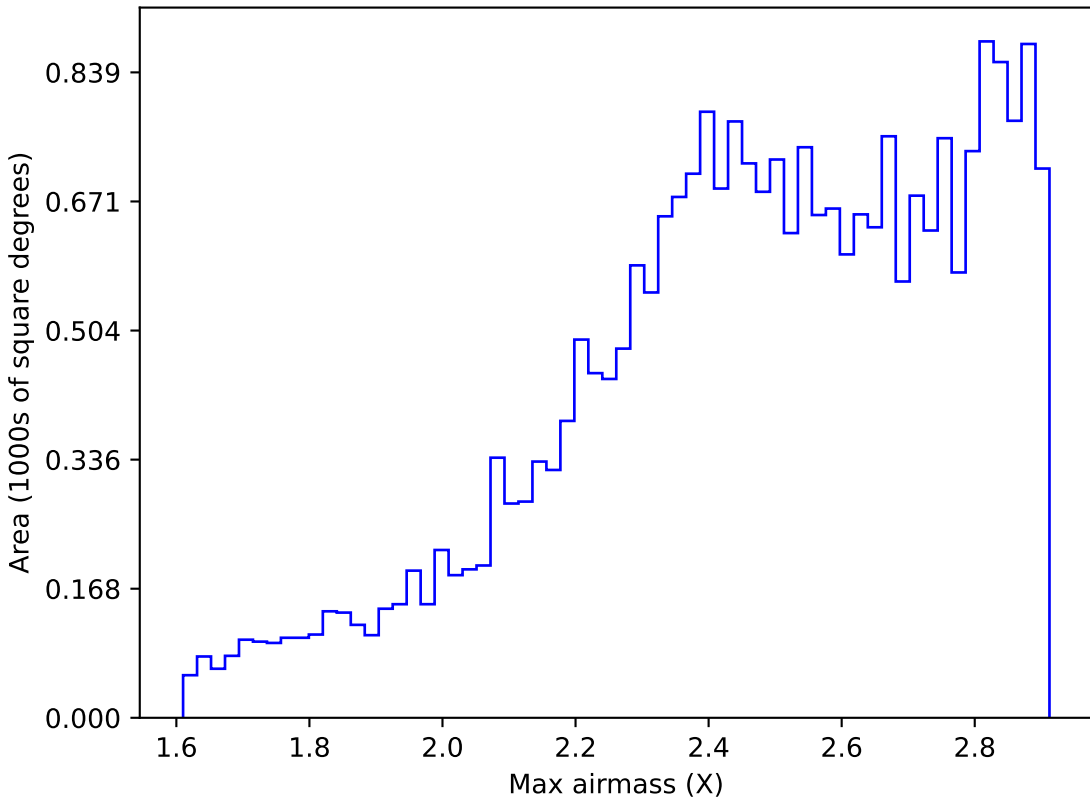
weather_cloudso2v3.4_10yrs All sky z band: Max airmass
