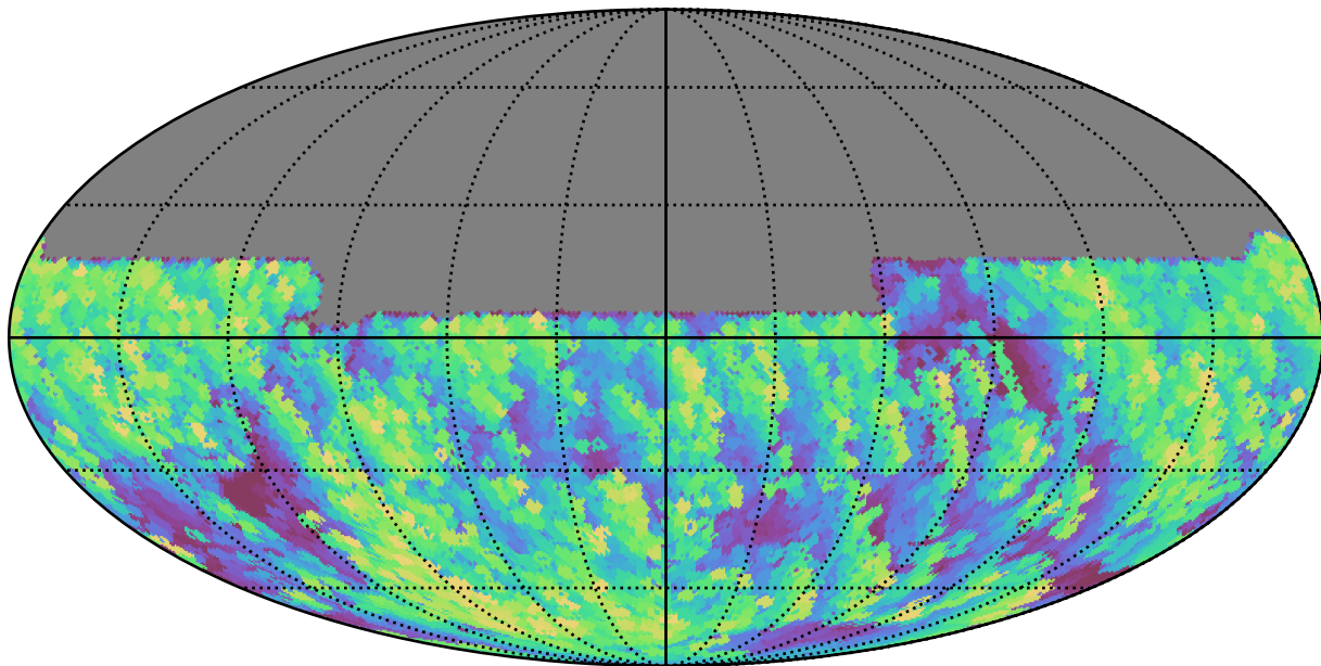
weather_cloudso2v3.4_10yrs All sky y band: Max airmass
