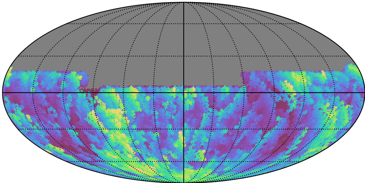
weather_cloudso2v3.4_10yrs All sky u band: Max airmass
