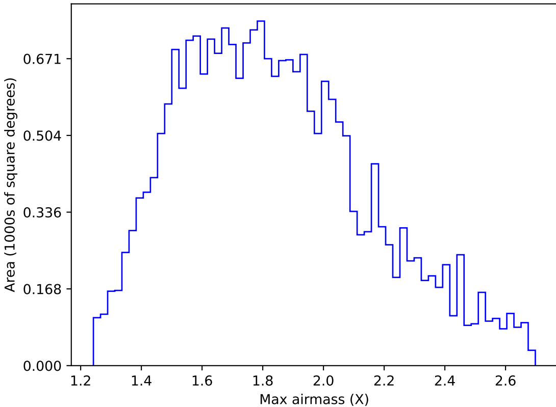
weather_cloudso2v3.4_10yrs All sky u band: Max airmass
