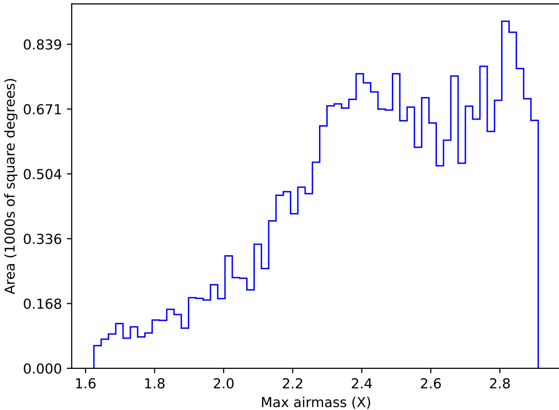
weather_cloudso2v3.4_10yrs All sky i band: Max airmass
