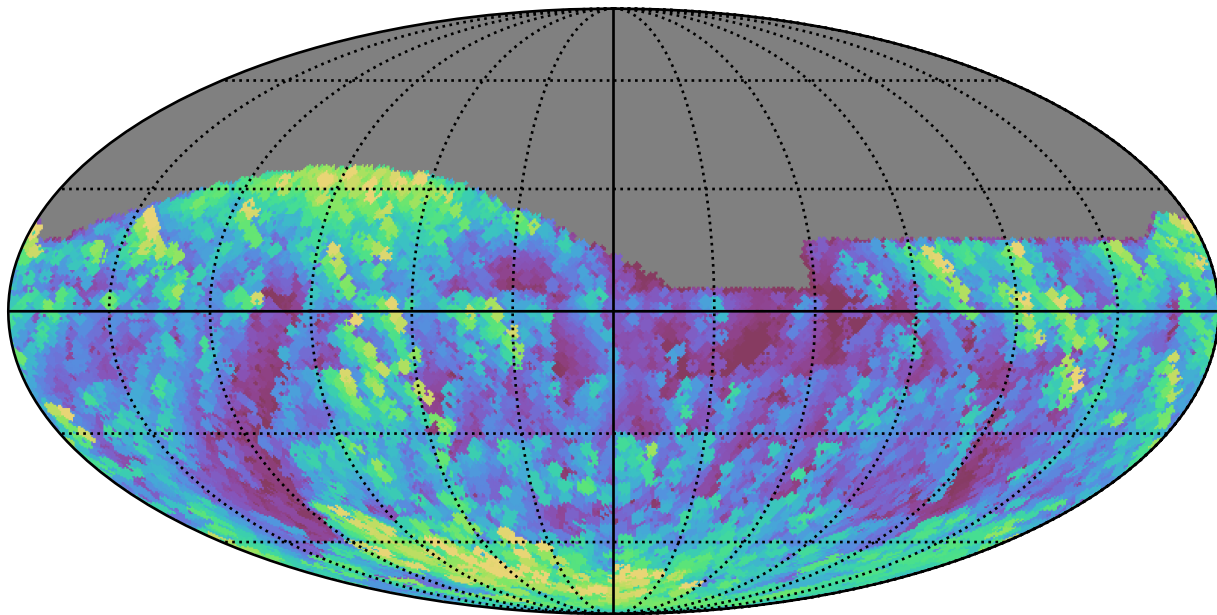
weather_cloudso2v3.4_10yrs All sky g band: Max airmass
