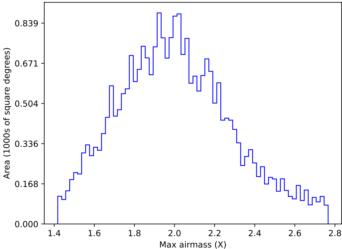
weather_cloudso2v3.4_10yrs All sky g band: Max airmass
