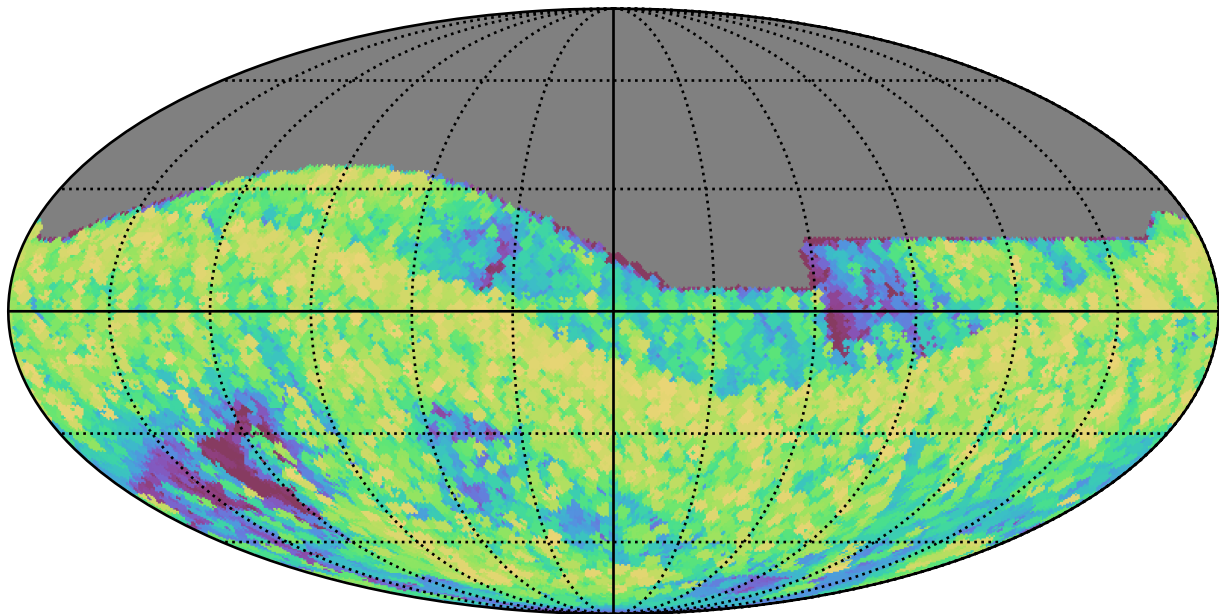
weather_cloudso2v3.4_10yrs All sky all bands: Max airmass
