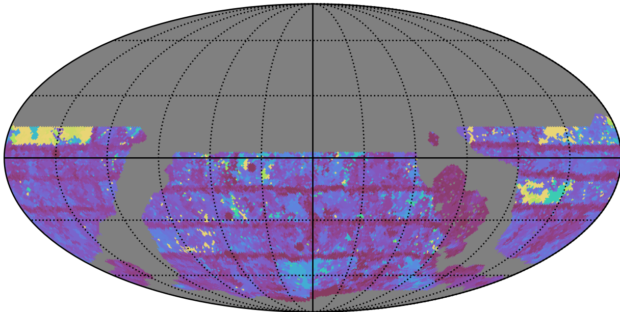
weather_cloudso2v3.4_10yrs WFD z band: Max Inter-Night Gap
