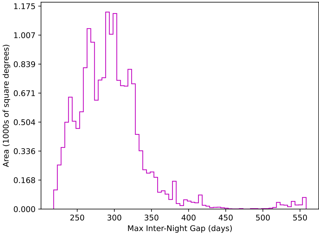
weather_cloudso2v3.4_10yrs WFD z band: Max Inter-Night Gap
