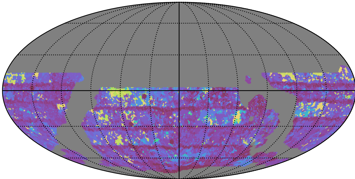
weather_cloudso2v3.4_10yrs WFD y band: Max Inter-Night Gap
