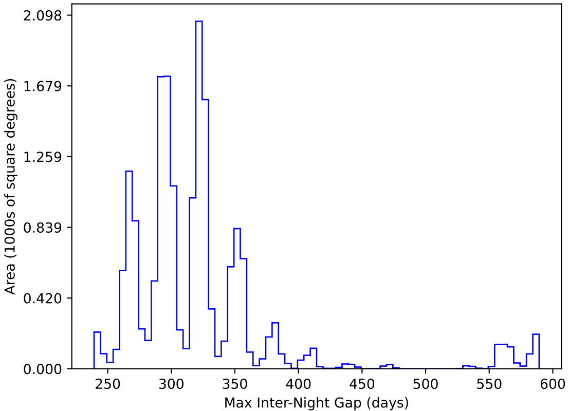
weather_cloudso2v3.4_10yrs WFD y band: Max Inter-Night Gap
