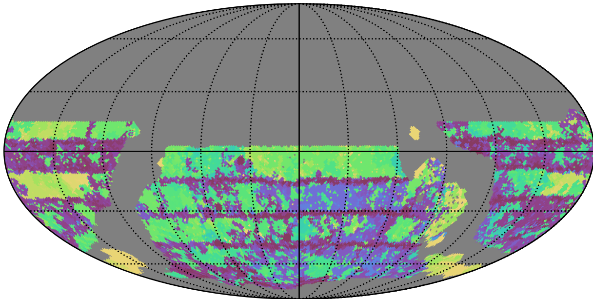
weather_cloudso2v3.4_10yrs WFD u band: Max Inter-Night Gap
