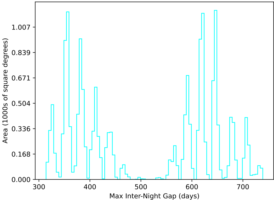
weather_cloudso2v3.4_10yrs WFD u band: Max Inter-Night Gap
