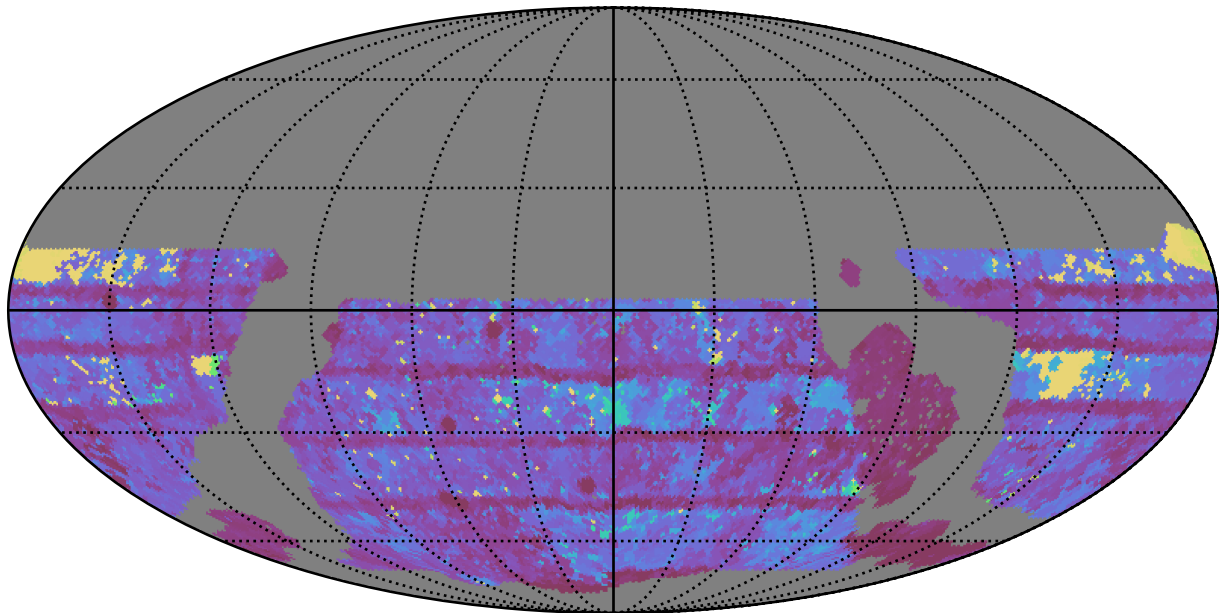
weather_cloudso2v3.4_10yrs WFD r band: Max Inter-Night Gap
