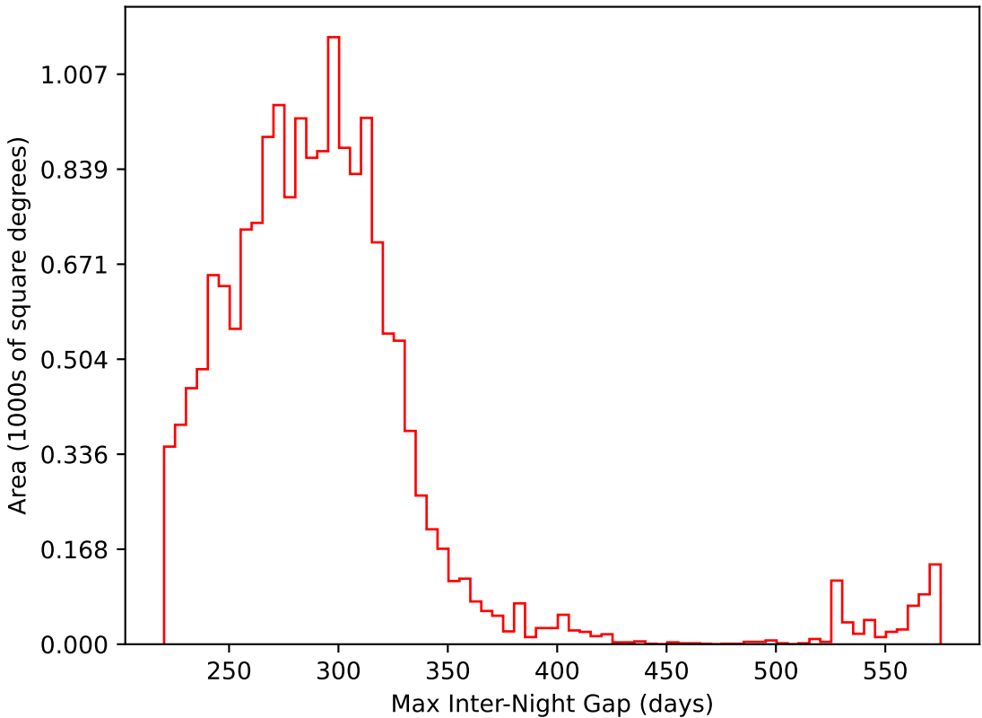
weather_cloudso2v3.4_10yrs WFD i band: Max Inter-Night Gap
