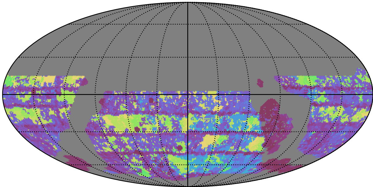
weather_cloudso2v3.4_10yrs WFD g band: Max Inter-Night Gap
