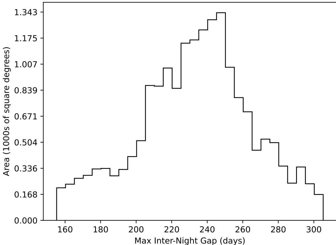
weather_cloudso2v3.4_10yrs WFD all bands: Max Inter-Night Gap
