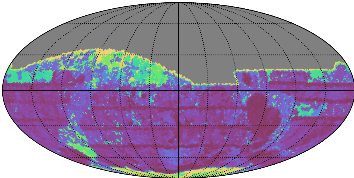
weather_cloudso2v3.4_10yrs All sky z band: Max Inter-Night Gap
