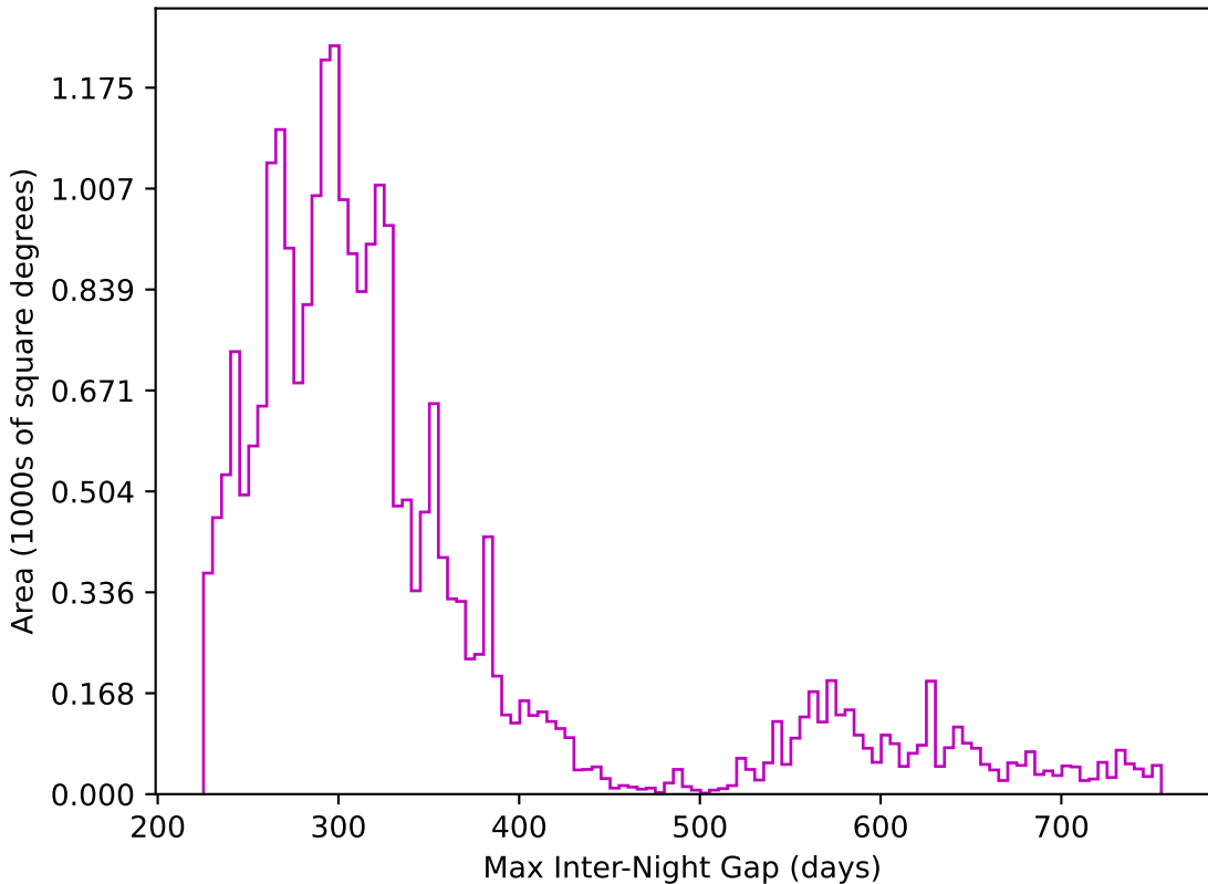
weather_cloudso2v3.4_10yrs All sky z band: Max Inter-Night Gap
