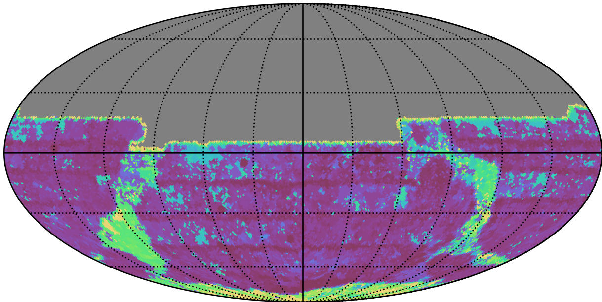
weather_cloudso2v3.4_10yrs All sky y band: Max Inter-Night Gap
