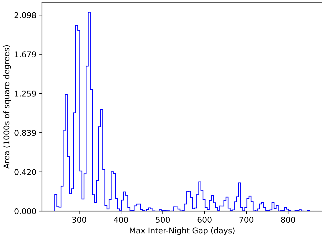
weather_cloudso2v3.4_10yrs All sky y band: Max Inter-Night Gap
