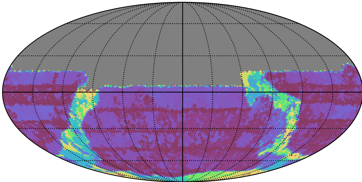
weather_cloudso2v3.4_10yrs All sky u band: Max Inter-Night Gap
