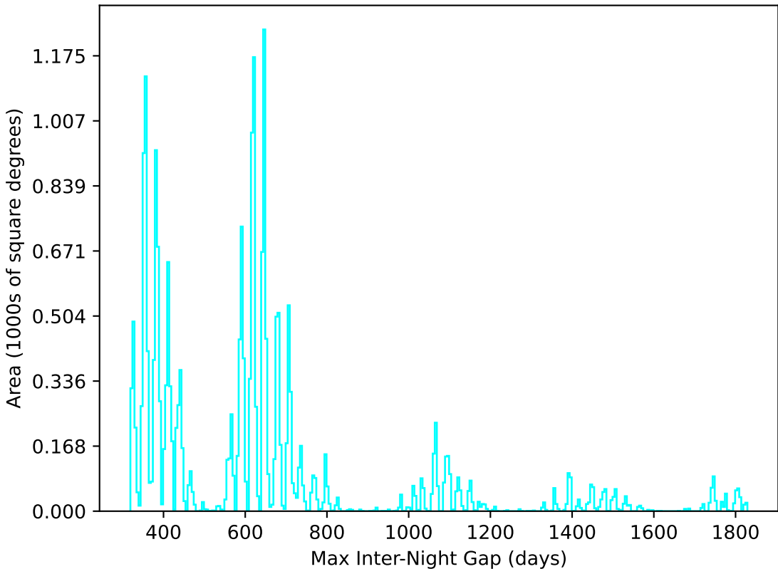
weather_cloudso2v3.4_10yrs All sky u band: Max Inter-Night Gap
