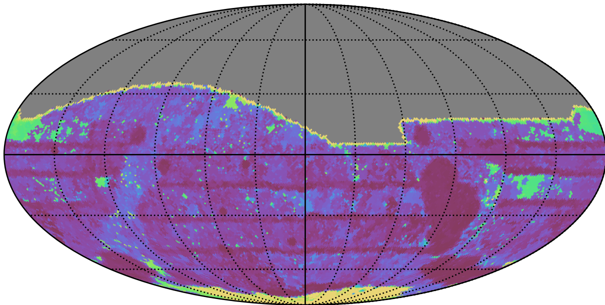
weather_cloudso2v3.4_10yrs All sky r band: Max Inter-Night Gap
