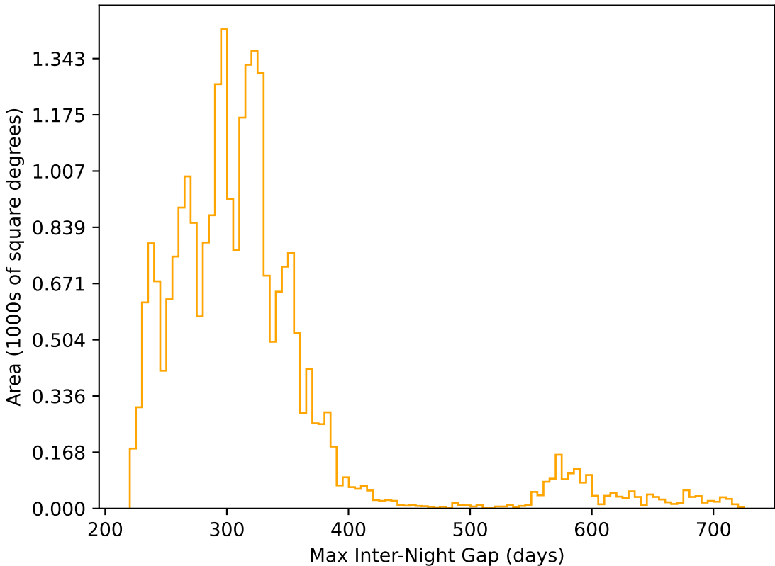
weather_cloudso2v3.4_10yrs All sky r band: Max Inter-Night Gap
