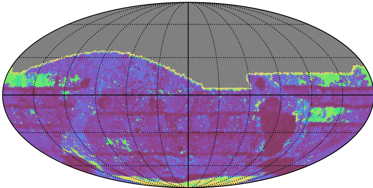
weather_cloudso2v3.4_10yrs All sky i band: Max Inter-Night Gap
