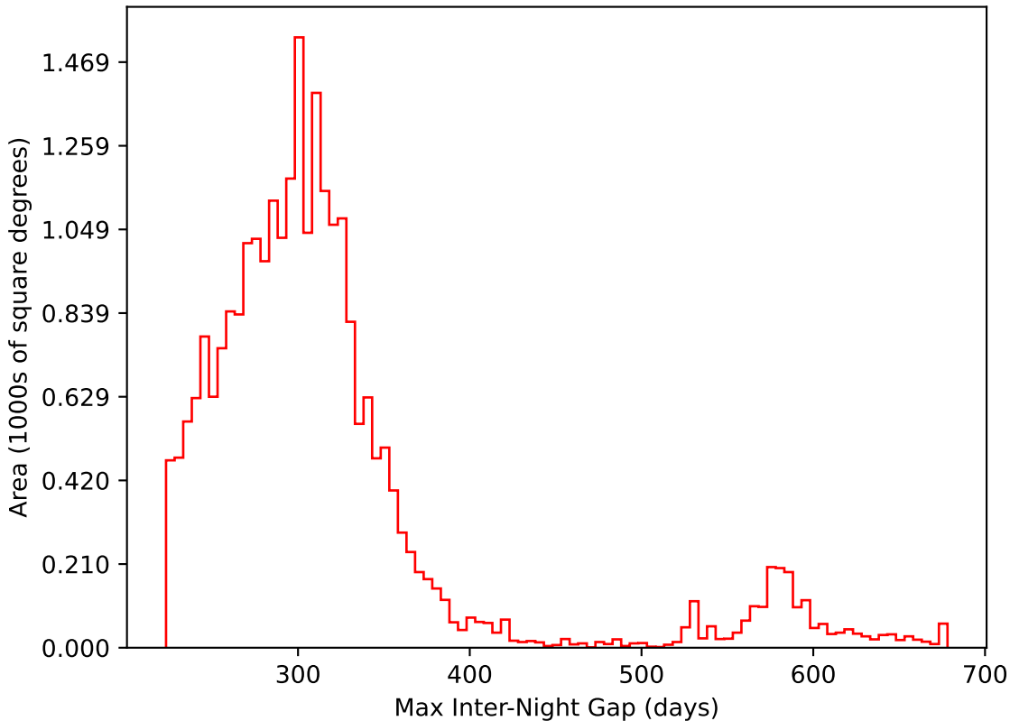
weather_cloudso2v3.4_10yrs All sky i band: Max Inter-Night Gap
