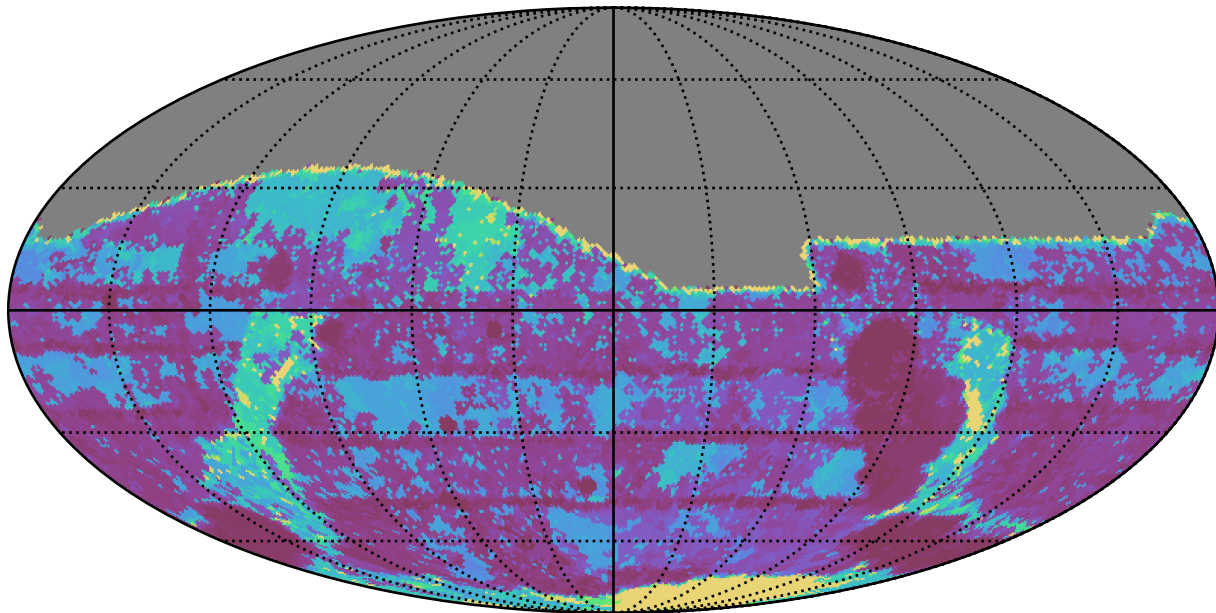
weather_cloudso2v3.4_10yrs All sky g band: Max Inter-Night Gap
