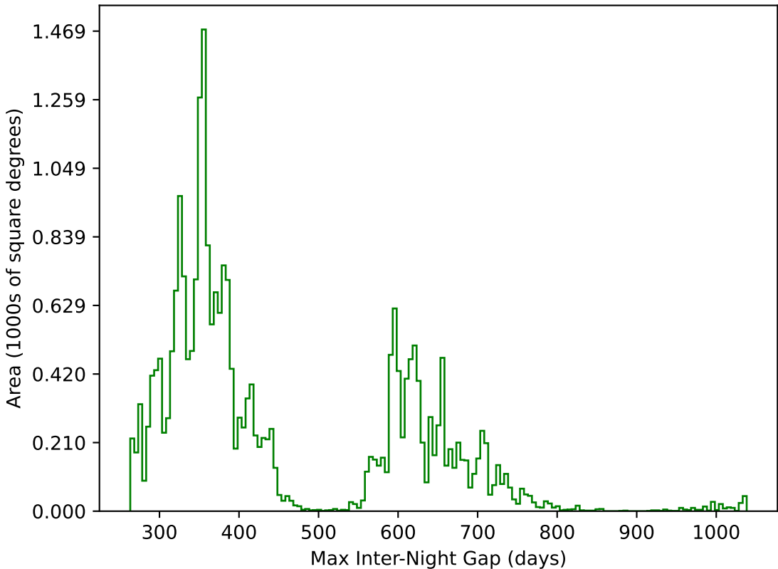
weather_cloudso2v3.4_10yrs All sky g band: Max Inter-Night Gap
