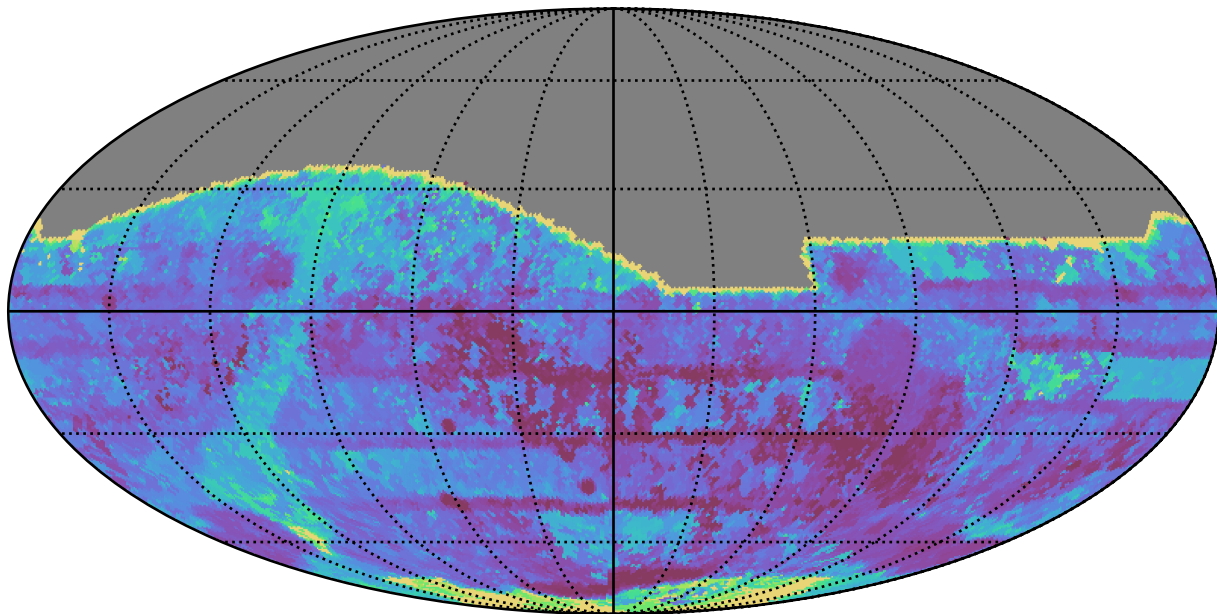
weather_cloudso2v3.4_10yrs All sky all bands: Max Inter-Night Gap
