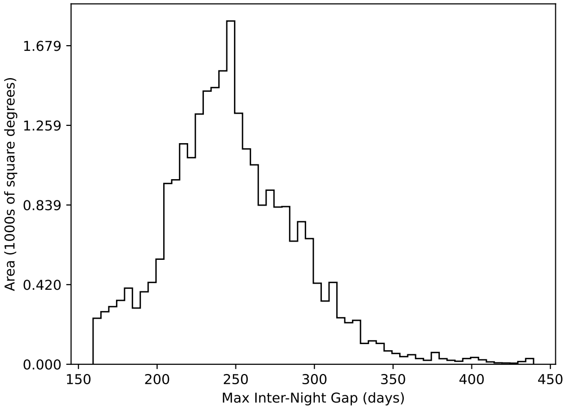
weather_cloudso2v3.4_10yrs All sky all bands: Max Inter-Night Gap
