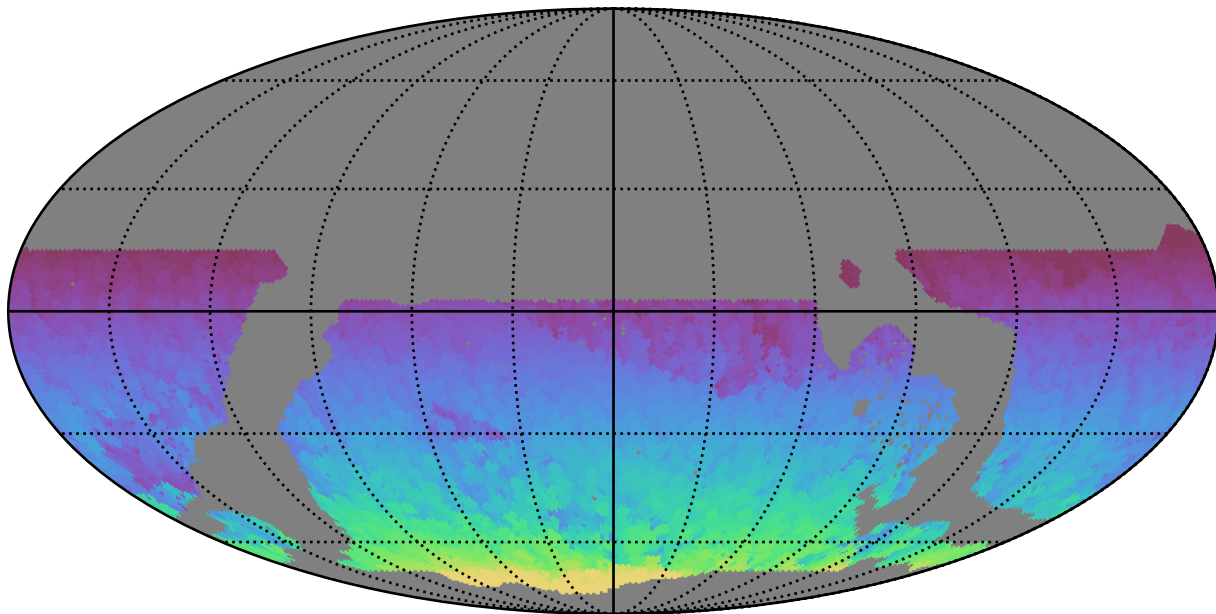
weather_cloudso2v3.4_10yrs WFD all bands: Max HA
