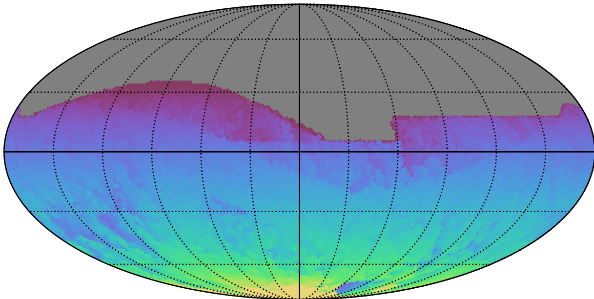
weather_cloudso2v3.4_10yrs All sky all bands: Max HA
