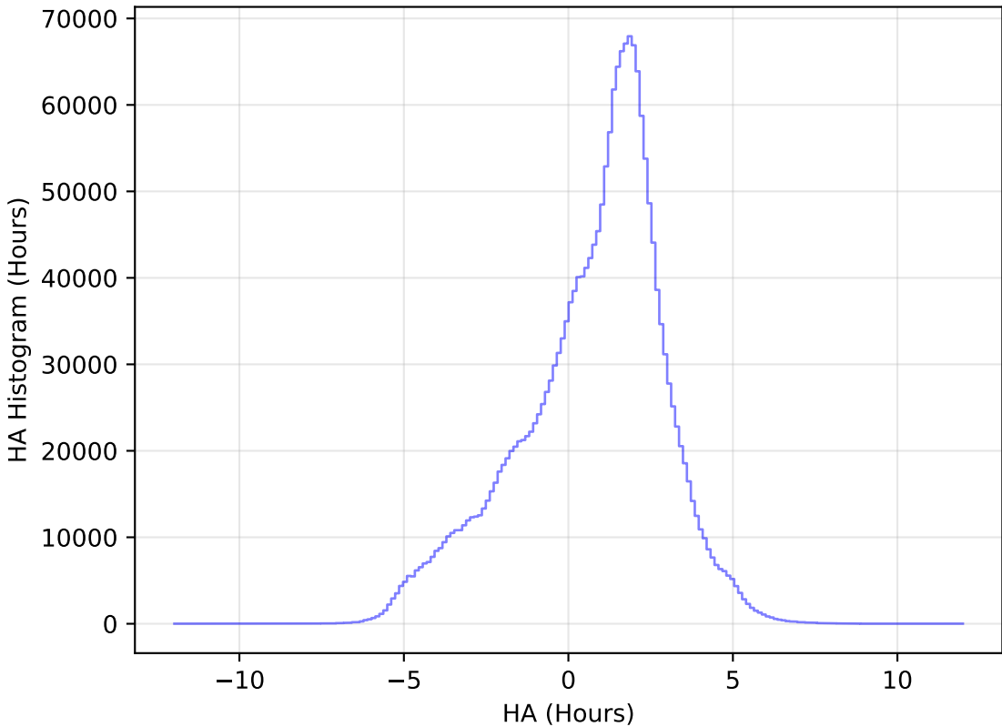
weather_cloudso2v3.4_10yrs All sky all bands: HA Histogram
