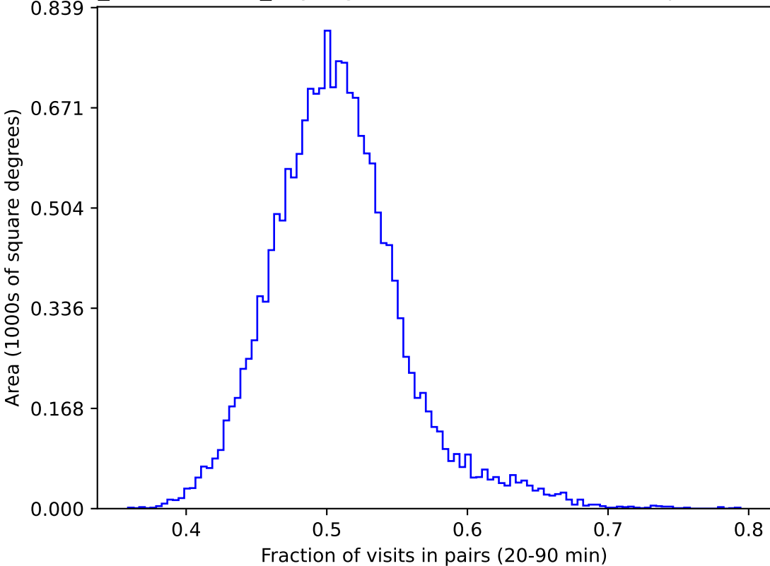
weather_cloudso2v3.4_10yrs gri WFD: Fraction of visits in pairs (20-90 min)
