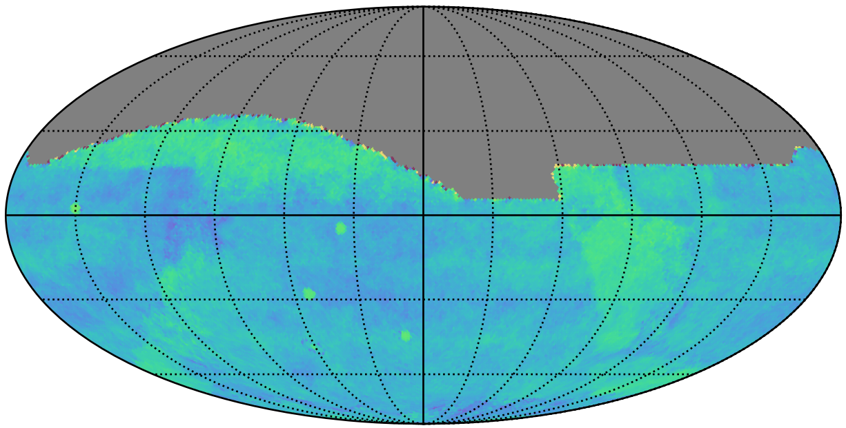
weather_cloudso2v3.4_10yrs gri All sky: Fraction of visits in pairs (20-90 min)
