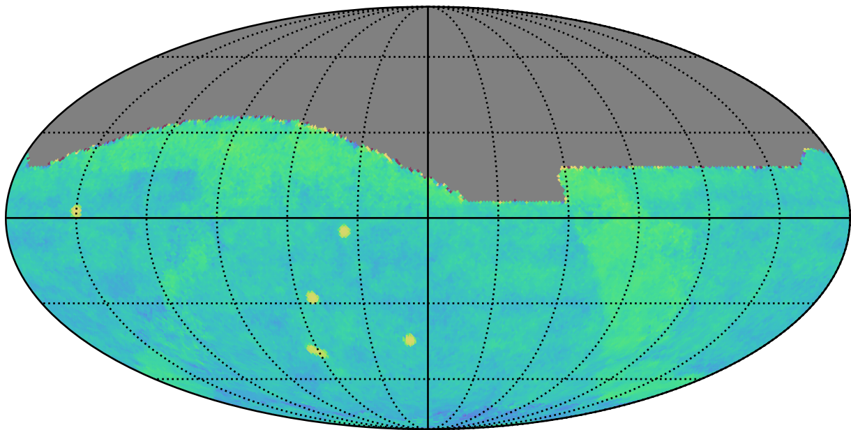
weather_cloudso2v3.4_10yrs gri All sky: Fraction of visits in pairs (10-60 min)
