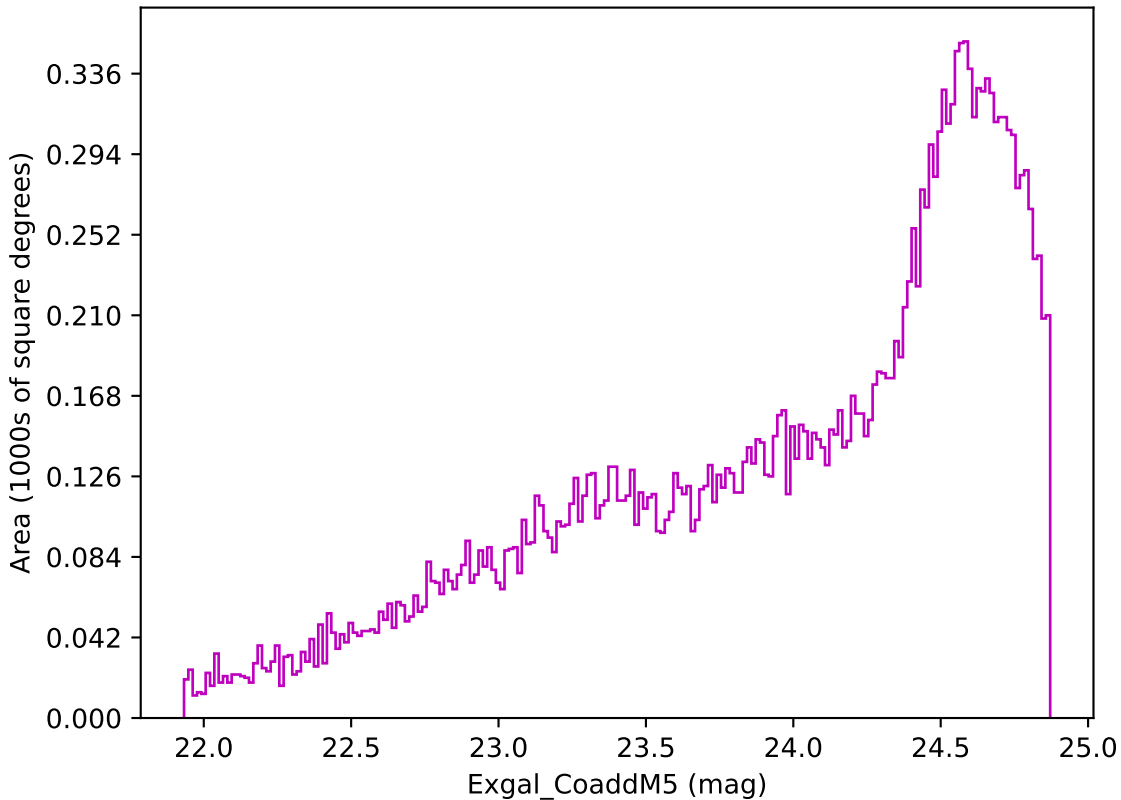
weather_cloudso2v3.4_10yrs Yr 3-4 z band: Exgal_CoaddM5
