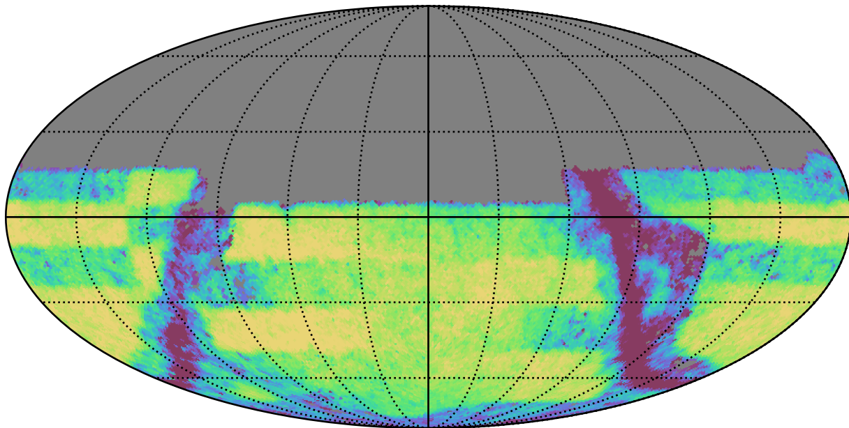
weather_cloudso2v3.4_10yrs Yr 3-4 y band: Exgal_CoaddM5
