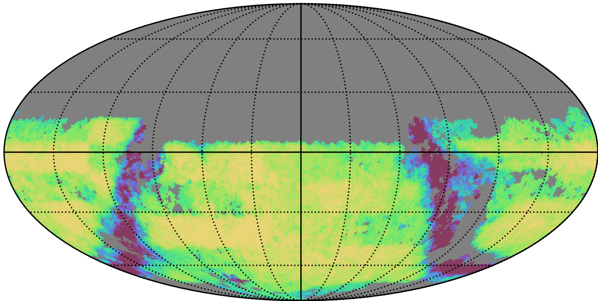
weather_cloudso2v3.4_10yrs Yr 3-4 u band: Exgal_CoaddM5
