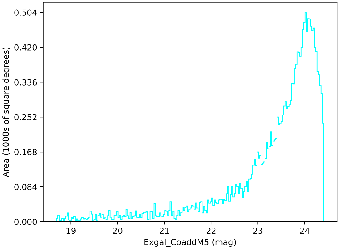
weather_cloudso2v3.4_10yrs Yr 3-4 u band: Exgal_CoaddM5
