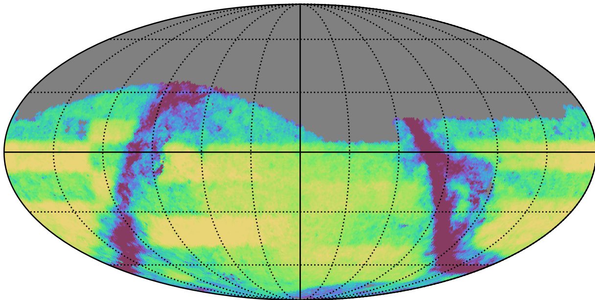
weather_cloudso2v3.4_10yrs Yr 3-4 r band: Exgal_CoaddM5
