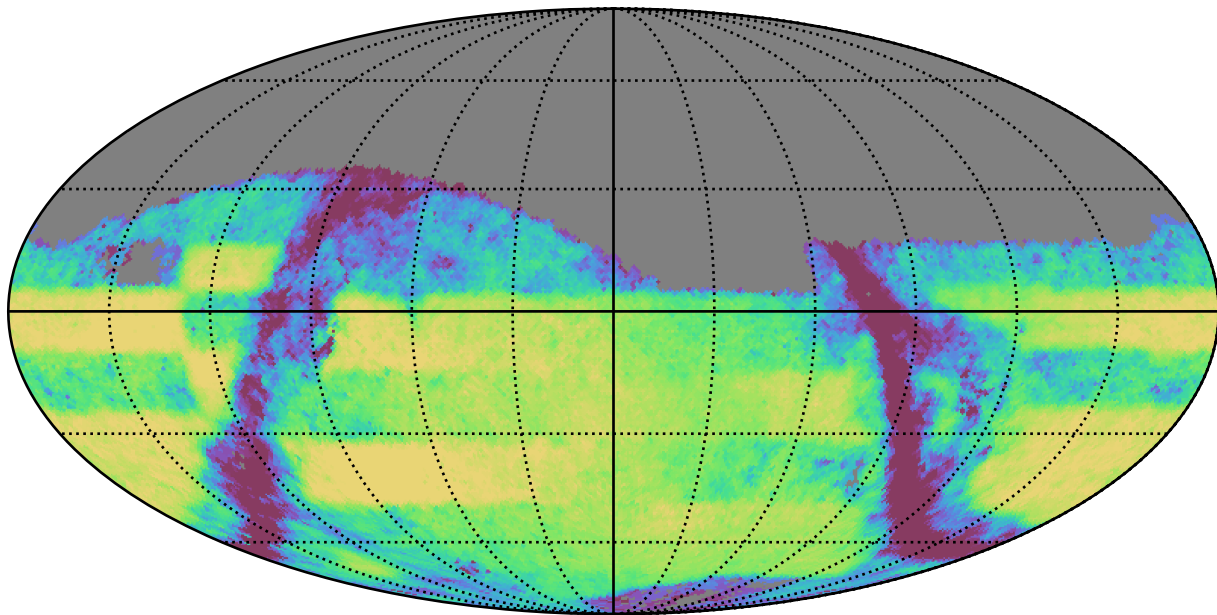
weather_cloudso2v3.4_10yrs Yr 3-4 i band: Exgal_CoaddM5
