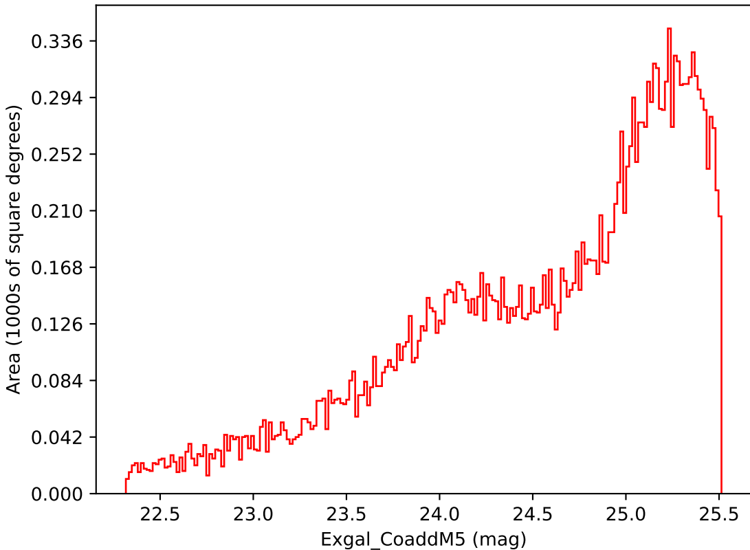
weather_cloudso2v3.4_10yrs Yr 3-4 i band: Exgal_CoaddM5
