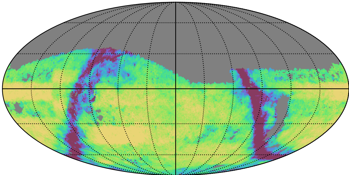
weather_cloudso2v3.4_10yrs Yr 3-4 g band: Exgal_CoaddM5
