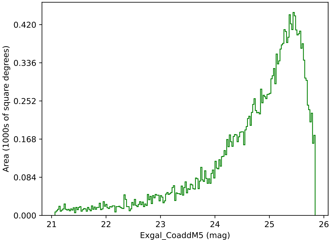
weather_cloudso2v3.4_10yrs Yr 3-4 g band: Exgal_CoaddM5
